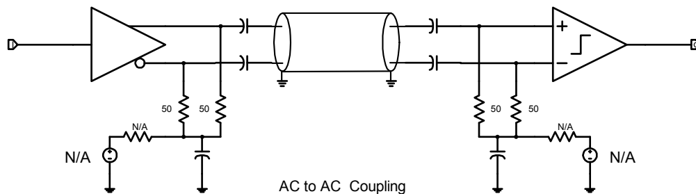
Figure 69 – Common mode biasing for Gen1x, Gen2i, and Gen2x
