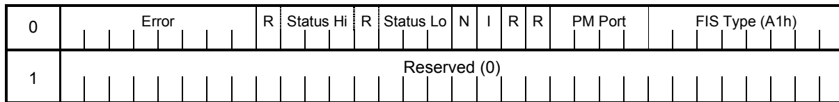
Figure 160 – Set Device Bit - Device to Host FIS layout
