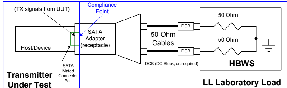
Figure 105 – Differential Voltage Amplitude Measurement
