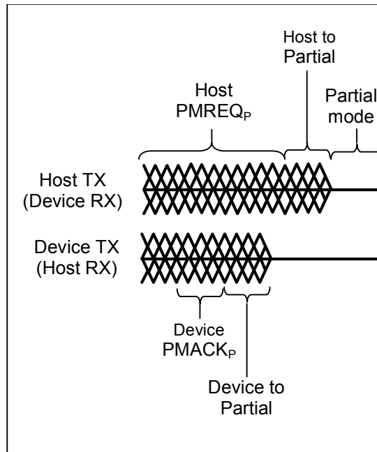
Figure 146 – PHYRDY to Partial/Slumber - Host initiated
