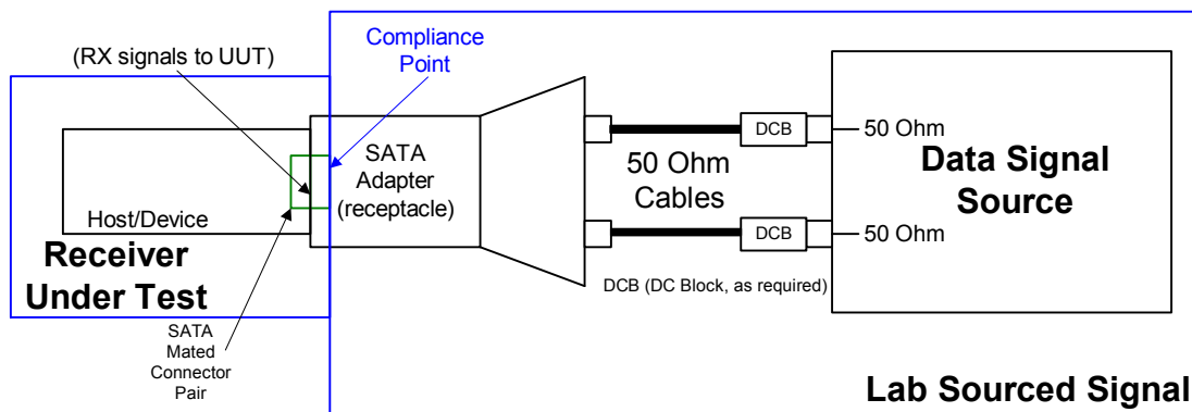
Figure 112 – Receiver Amplitude Test
