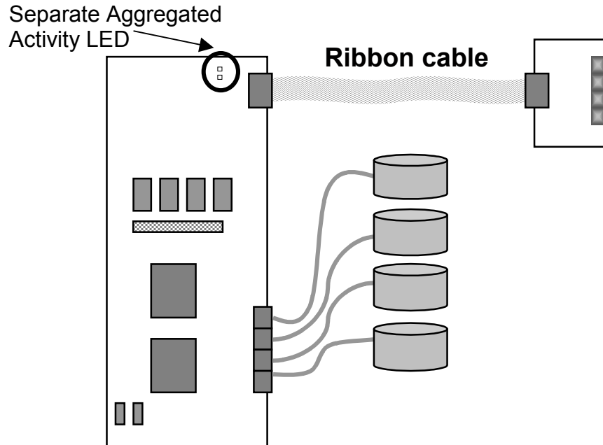
Figure 202 – Device Activity LEDs with Ribbon Cable
