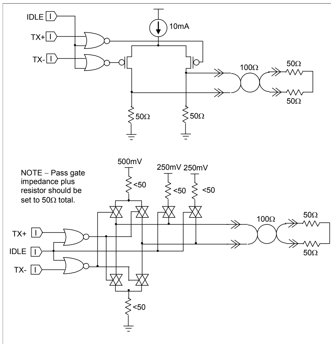
Figure 139 – Transmitter examples
