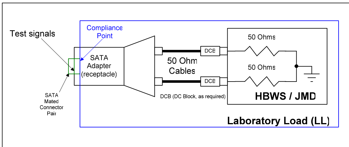
Figure 76 – LL Laboratory Load
