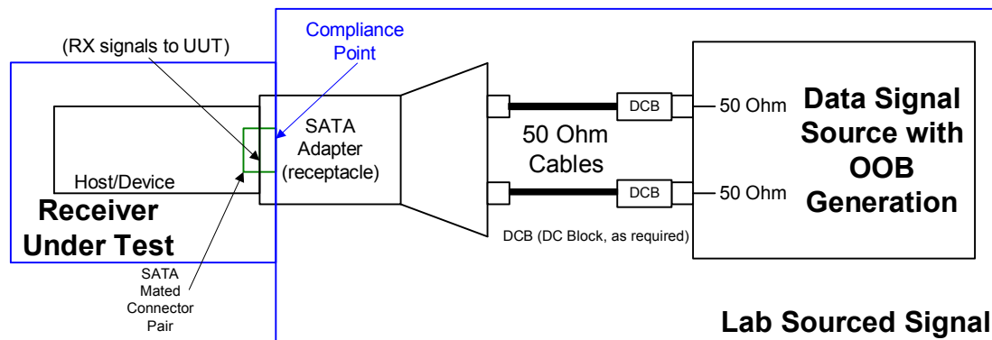
Figure 131 – Squelch Detector Threshold Test
