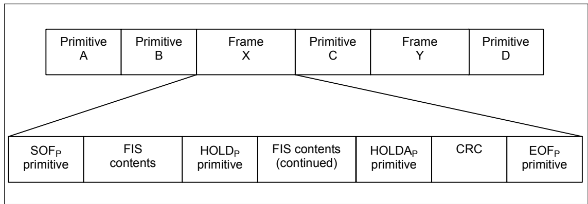
Figure 155 – Transmission structures
