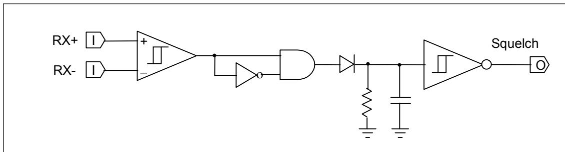
Figure 144 – Squelch detector
