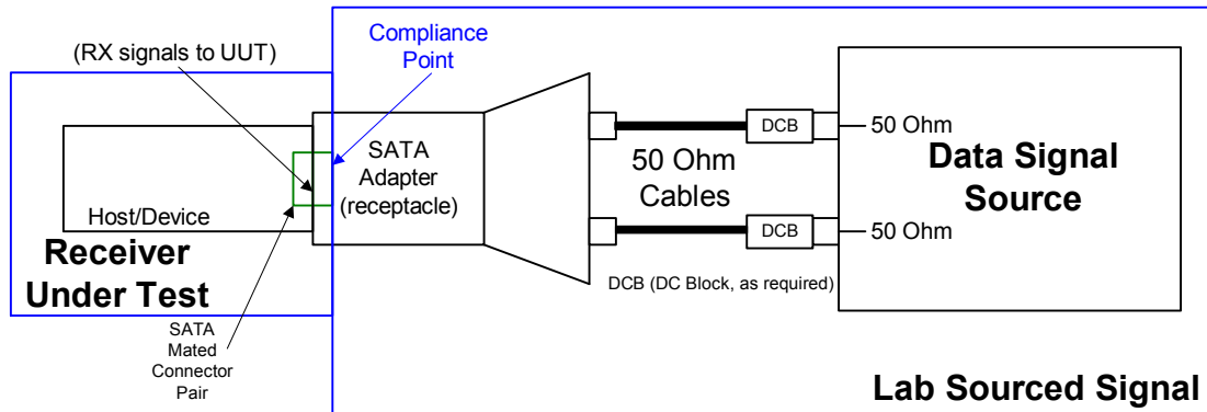
Figure 126 – Receiver Intra-pair Skew Test
