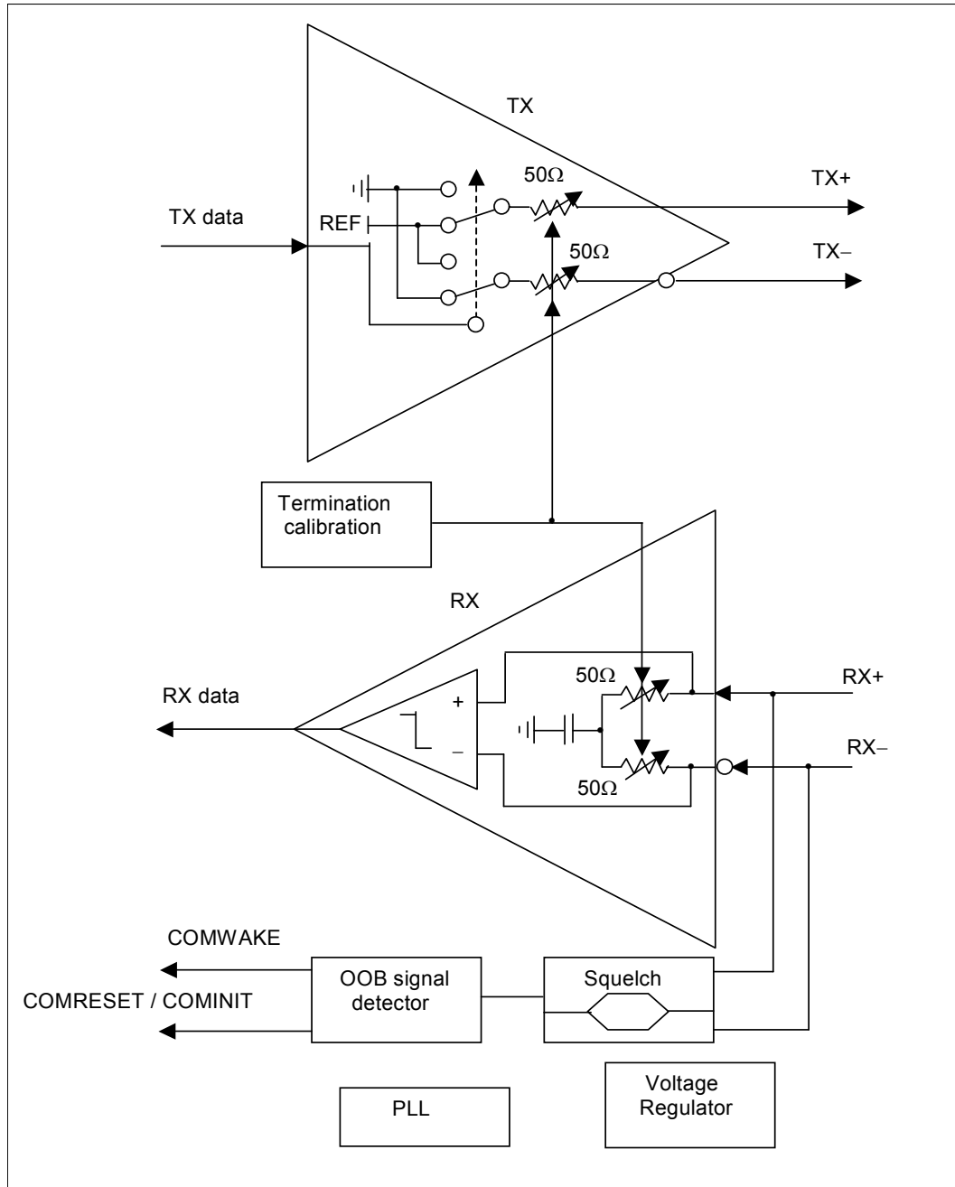
Figure 65 – Analog front end (AFE) block diagram
